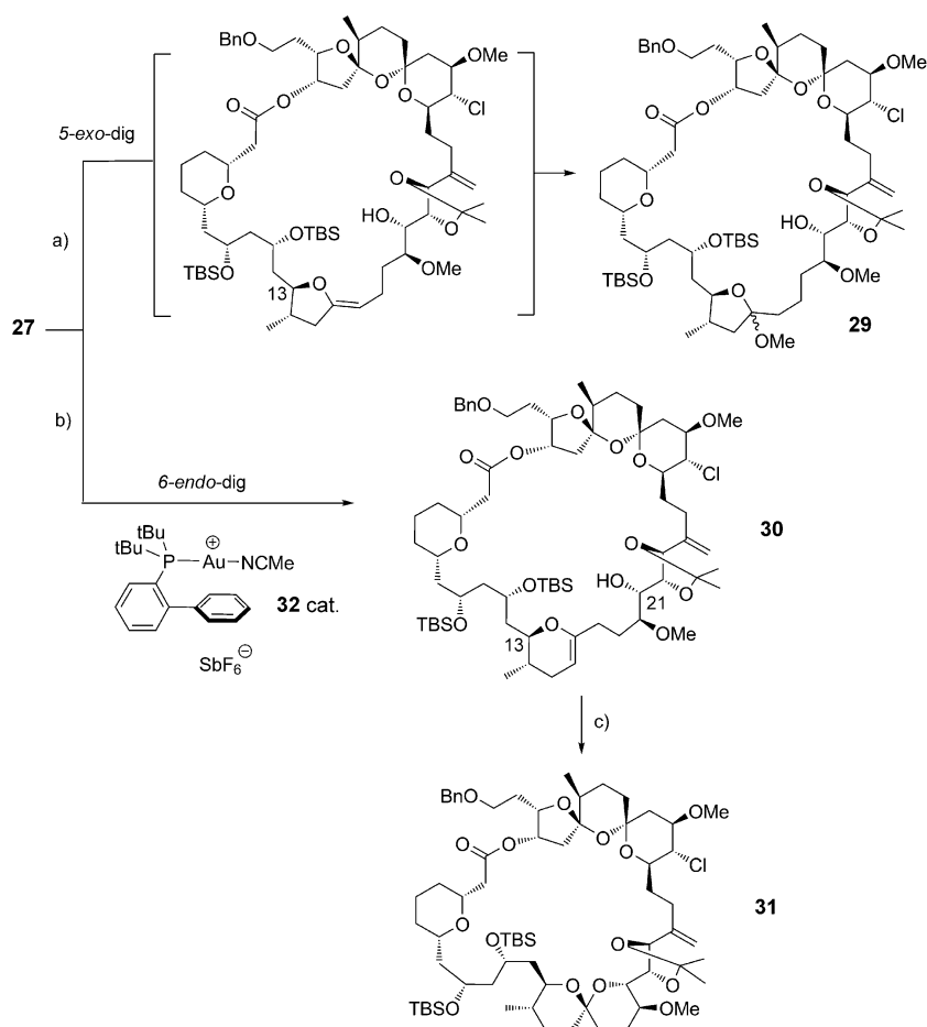
Scheme 5. a) AuCl-SMe 2 (10 mol %), CH 2 Cl 2 , then MeOH, PPTS cat., 36%, see text for details; b) 32 (10 mol %), CH 2 Cl 2 , 4 Å M.S., 62% (endo/exo = ca. 5:1); c) PPTS cat., toluene, 80 °C, 81%. PPTS = pyridinium p -toluenesulfonate.
