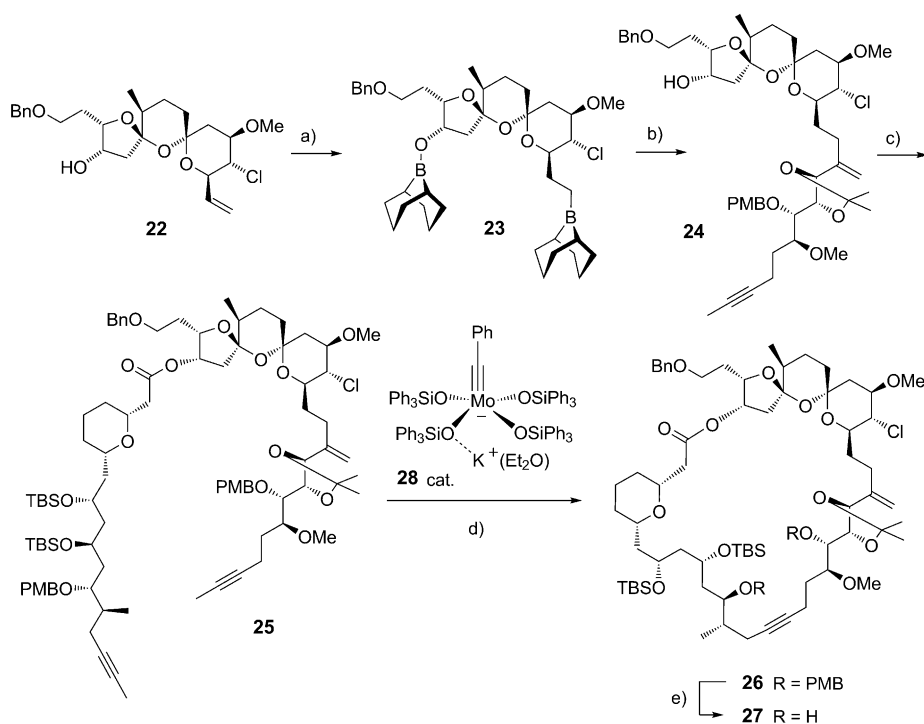
Scheme 4. a) 9-H-9-BBN dimer, THF; b) aq NaOH (1 M), [PdCl 2 (dppf)] (20 mol %), Ph 3 As (20 mol %), 21 , THF, 76%; c) 1. 9 , 2,4,6-trichlorobenzoyl chloride, Et 3 N, toluene, 0 °C; 2. 24 , DMAP, toluene, 0 °C → RT, 85%; d) 28 (8 mol %), 5 Å M.S., toluene, 87%; e) DDQ, CH 2 Cl 2 , 0 °C → RT, 91 %. 9-BBN = 9-borabicyclo[3.3.1]nonane, dppf = 1,1'-bis(diphenylphosphino)ferrocene, DMAP = 4-dimethylamino-pyridine; M.S. = molecular sieves.
